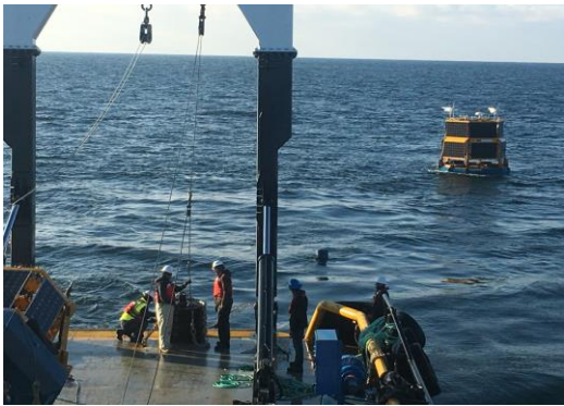
Floating LIDAR center of Empire Wind lease
